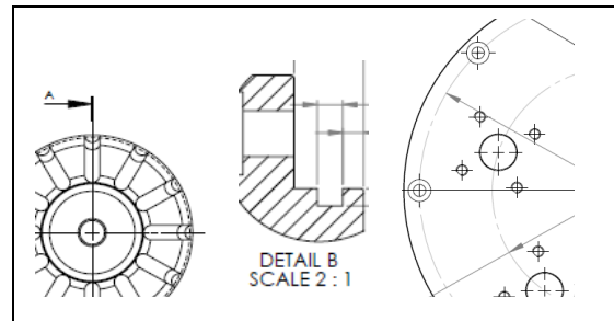
CAD Design, 3D models and Drawing.
